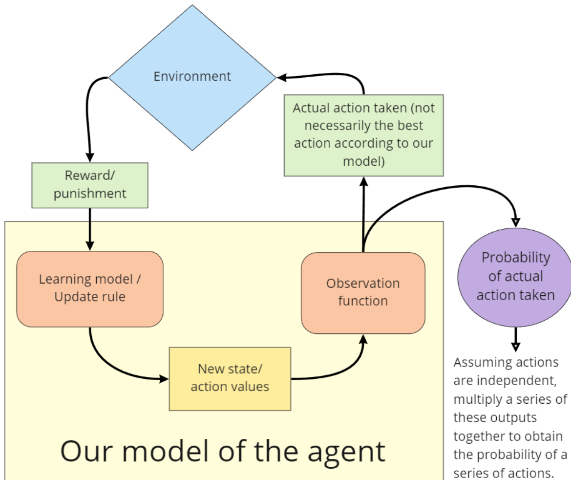
Figure 3.2: The observation function and learning model/update rule are both part of our model of the agent. To fit this model to data, we need to find the probability that the model would result in the chain of actions we have recorded. For each action, we calculate the probability that the model would choose that action given everything that has happened up to that point. Once we have probabilities for all the actions, we usually multiply those probabilities together under the assumption that the actions are independent.
